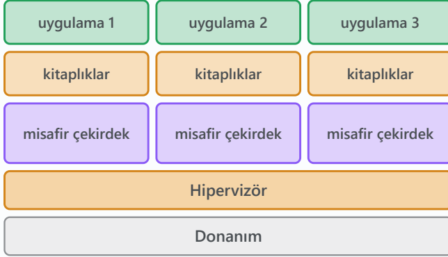
(a) sanal makineler
